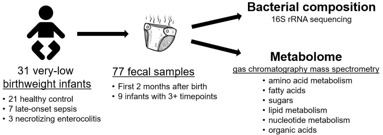
Figure 1. Study design schematic. Longitudinal fecal samples were collected over the first 75 days of life from very low birthweight infants in the NICU. Bacterial compositions and metabolomes were characterized.
